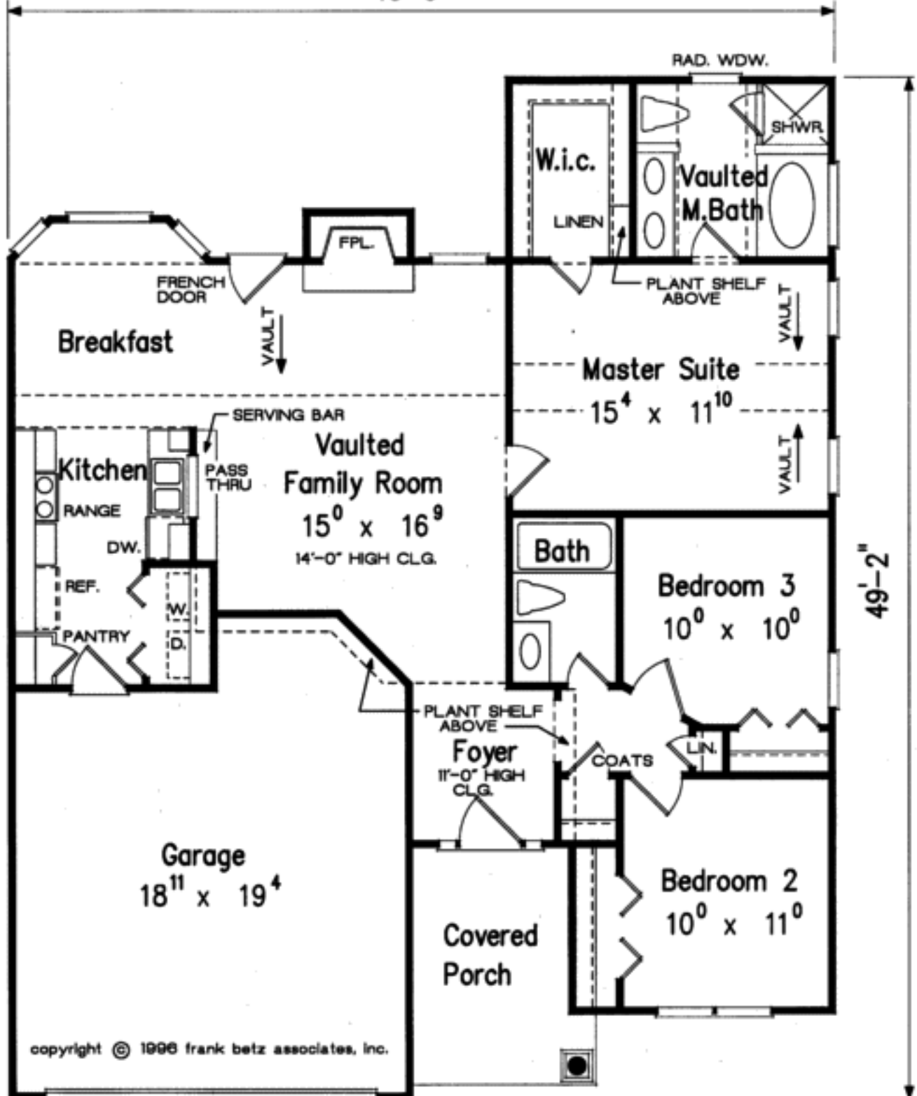
FLOOR PLAN
